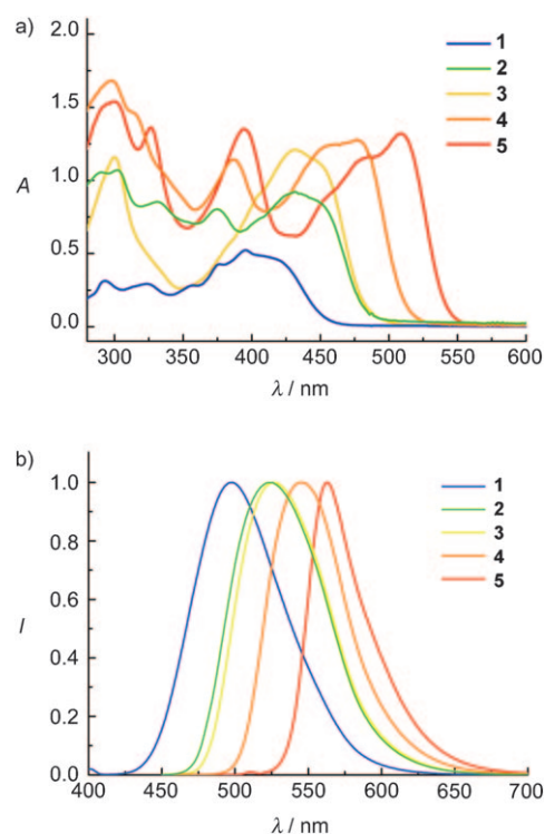
Figure 2. a) UV/Vis spectra of 1–5 in CH 2 Cl 2 . b) Normalized fluorescence spectra of 1–5 in CH 2 Cl 2 .
